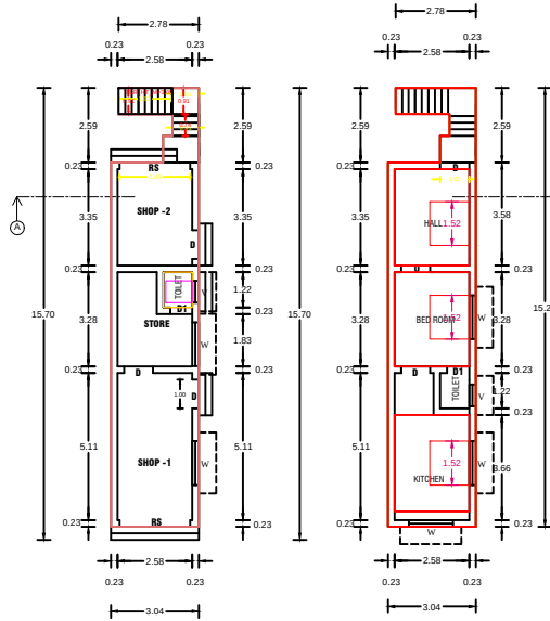
EXG.GROUND FLOOR PLAN
