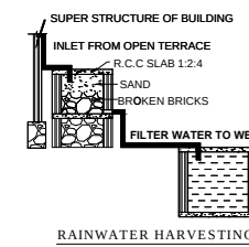
RAINWATER HARVESTING
