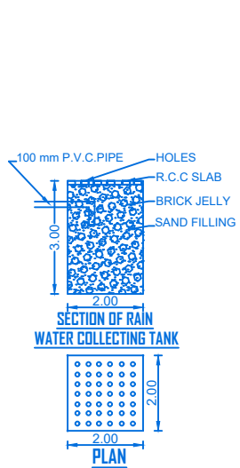
PLAN
