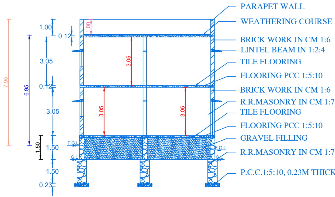
SECTION ON "V-B"
