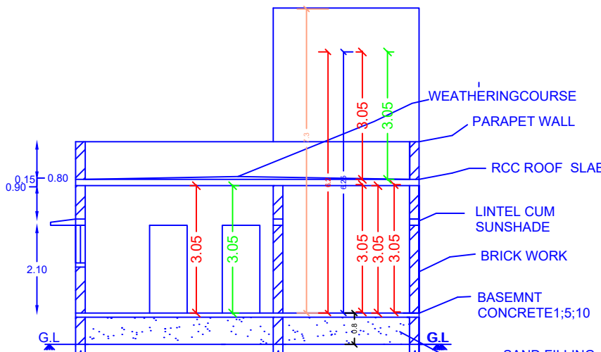
SECTION AB
