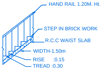
STAIR DETAIL
