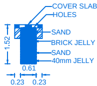
SECTION OF RAIN WATER COLLECTION TANK
