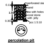
percolation pit
