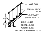
STAIR DETAILS
