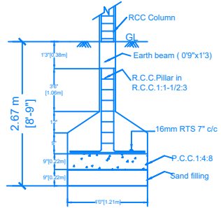
FOUNDATION DETAILS
