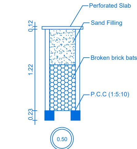
RAIN WATER COLLECTION WELL
