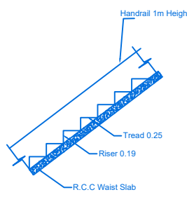
STAIR DETAILS
