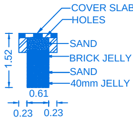
SECTION OF RAIN WATER COLLECTION TANK
