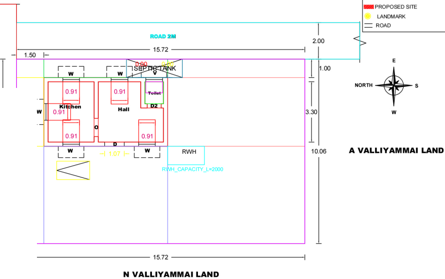
SITE PLAN FOR THE PROPOSAL
