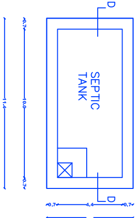
PLAN OF SEPTIC TANK SCALE 1"=2'0"
