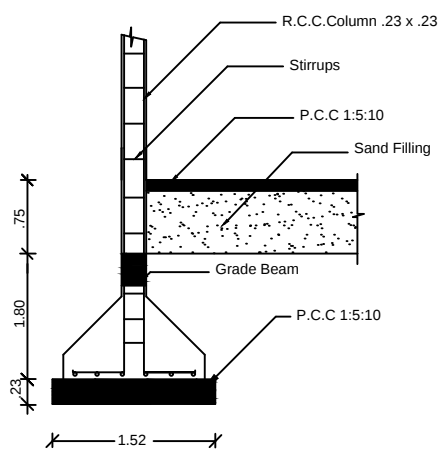
COLUMN DETAIL
