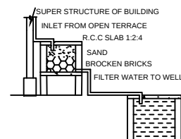
RAINWATER HARVESTING
