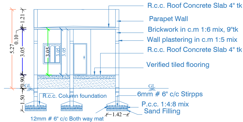
SECTION NN
