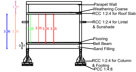
SECTION AB
