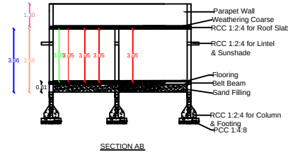
SECTION AB
