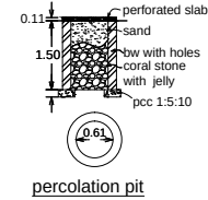
percolation pit
