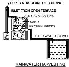
RAINWATER HARVESTING
