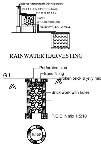
PERCOLATION PIT FOR 30 Sq. m. (NOT FOR SCALE)
