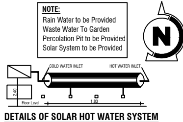
DETAILS OF SOLAR HOT WATER SYSTEM
