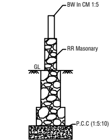
DETAILS OF RR MASONRY
