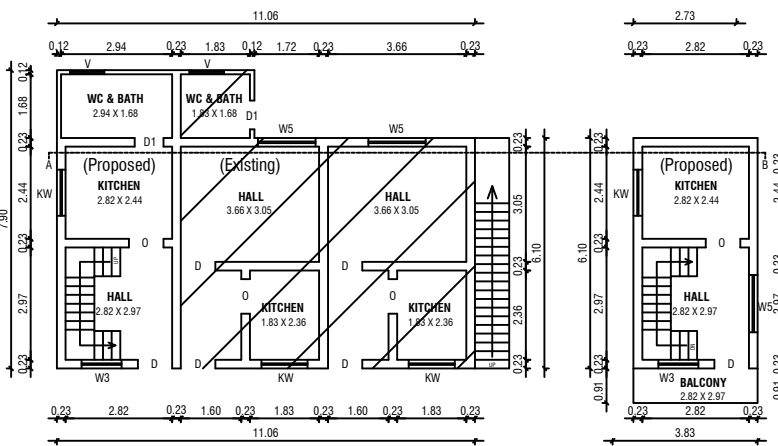
GROUND FLOOR PLAN (PROPOSED)
