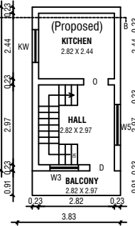
FIRST FLOOR PLAN (PROPOSED)
