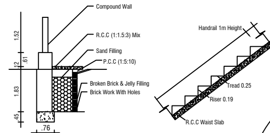
RAIN WATER HARVEST DETAILS
