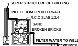
RAINWATER HARVESTING
