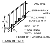
STAIR DETAILS
