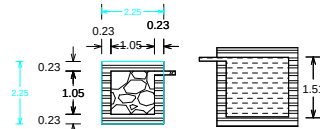
DETAILS OF FILTER BED & WELL
