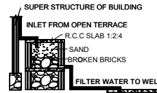
RAINWATER HARVESTING
