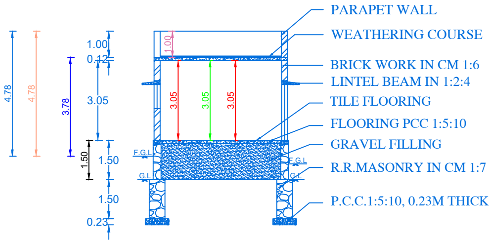
SECTION ON "V-B"
