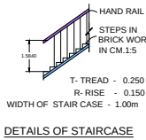
DETAILS OF STAIRCASE
