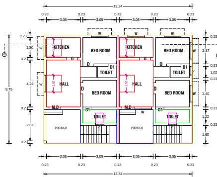
PLAN-1 & PLAN - 2
