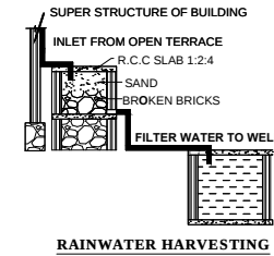
RAINWATER HARVESTING
