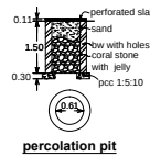
percolation pit
