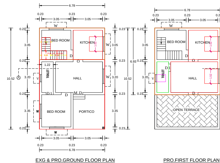
EXG & PRO.GROUND FLOOR PLAN
