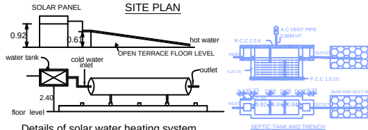
Details of solar water heating system
