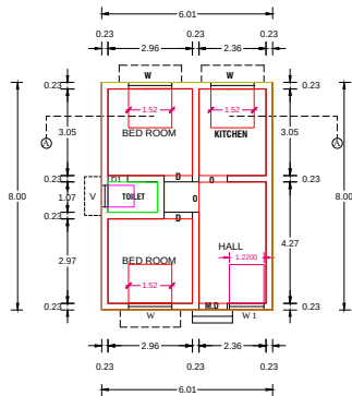
PLAN
