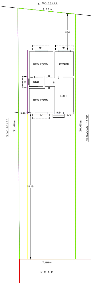
SITE PLAN
