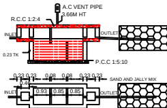
SEPTIC TANK AND TRENCH
