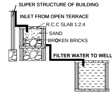
RAINWATER HARVESTING
