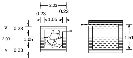
DETAILS OF FILTER BED & WELL
