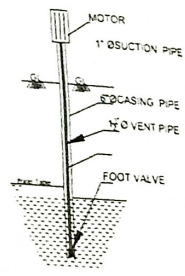
SEC. OF BOREWELL
