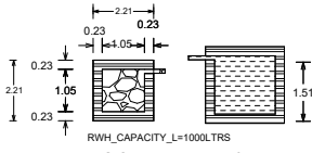
DETAILS OF FILTER BED & WELL
