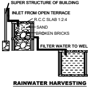
RAINWATER HARVESTING
