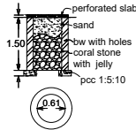
percolation pit
