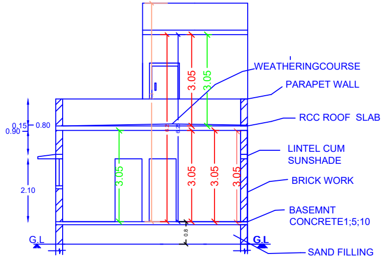
SECTION AB
