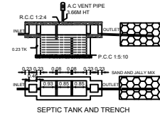
SEPTIC TANK AND TRENCH
