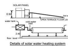
Details of solar water heating system
