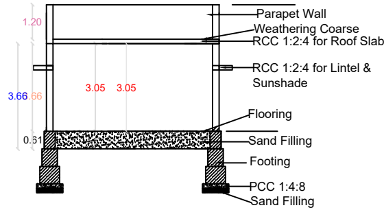
SECTION AB
