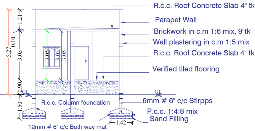
SECTION NN
