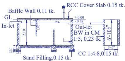
SECTION - SEPTIC TANK
