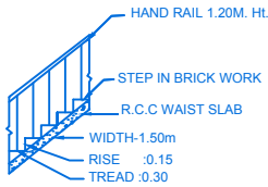
STAIR DETAIL
