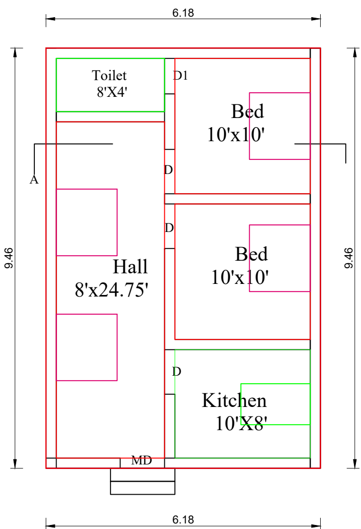
PLAN
