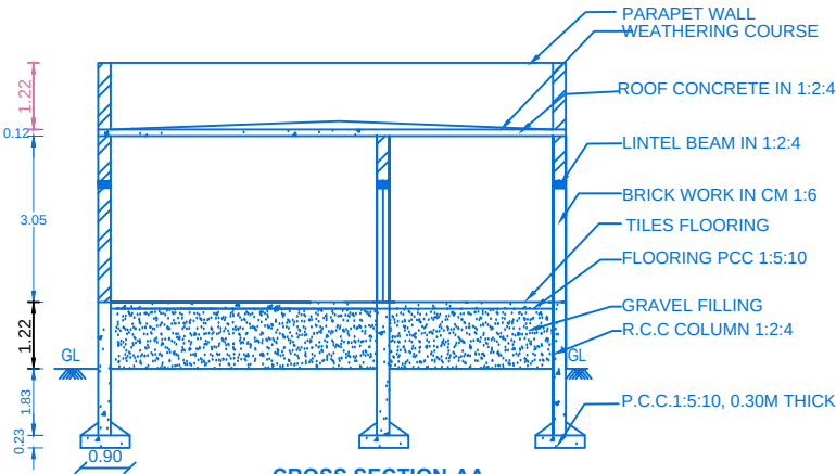
CROSS SECTION-AA
