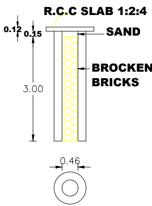
PERCOLATION PIT
