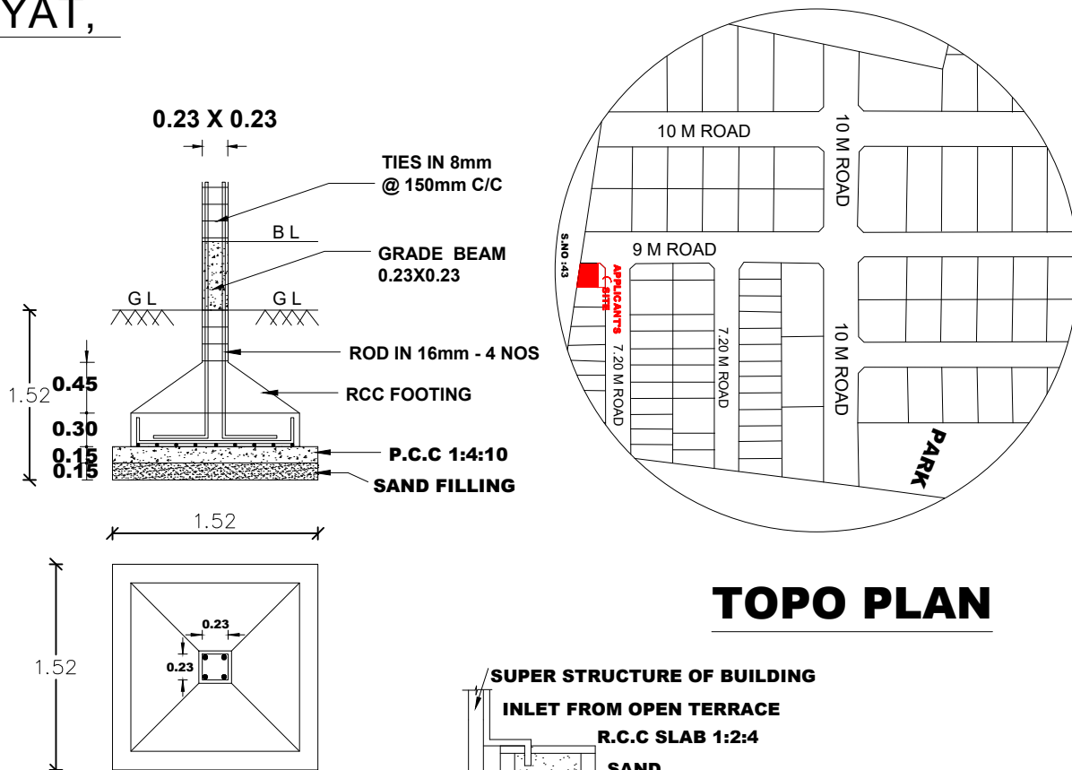
RCC COLUMN DETAILS
