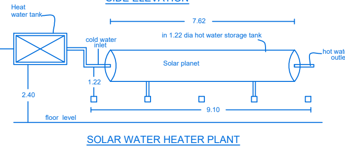
SOLAR WATER HEATER PLANT
