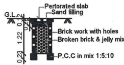
PERCOLATION PIT FOR 30 Sq. m. (Scale:- 1:50)
