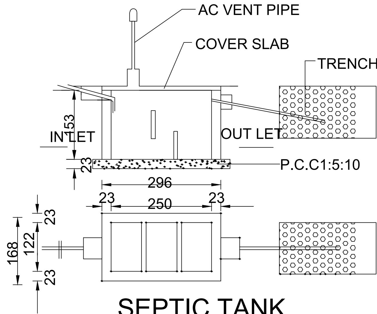
SEPTIC TANK
