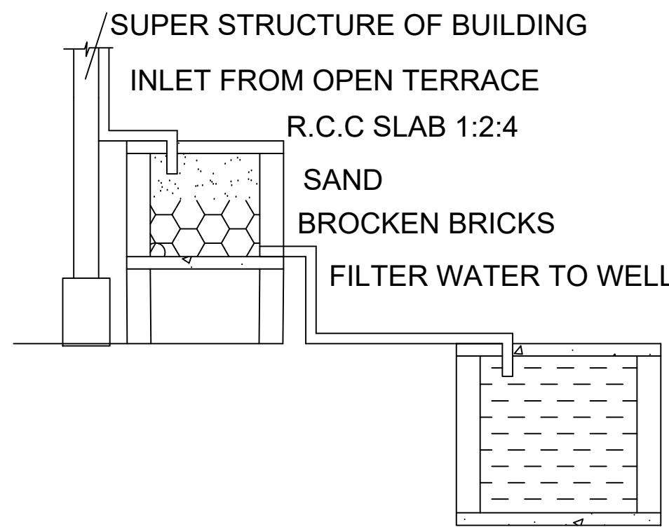
RAINWATER HARVESTING
