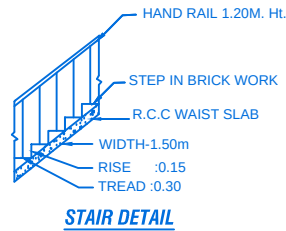
STAIR DETAIL
