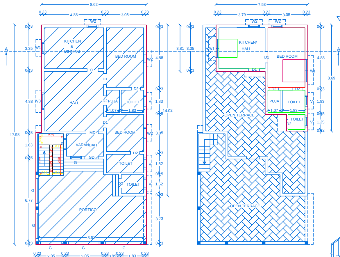
EXG.GROUND FLOOR PLAN
