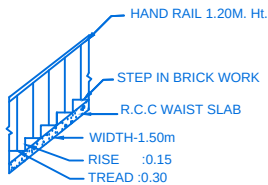
STAIR DETAIL
