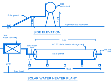
SIDE ELEVATION
