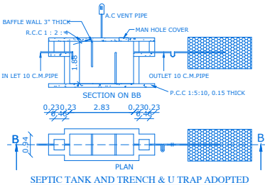
SEPTIC TANK AND TRENCH & U TRAP ADOPTED
