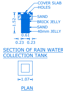
PLAN
