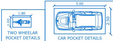
ALL DIMENSIONS ARE IN METRE SCALE 1:100
