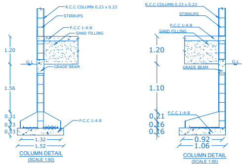
COLUMN DETAIL (SCALE 1:50)
