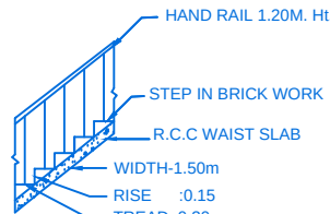
STAIR DETAIL
