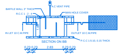
SECTION ON BB
