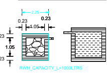
RAINWATER HARVESTING
