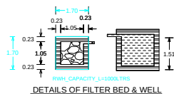
DETAILS OF FILTER BED & WELL
