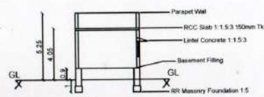
SECTION A-A VIEW
