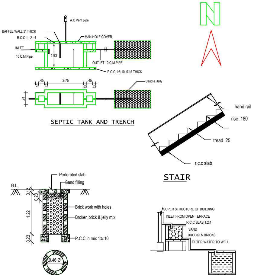
PERCOLATION PIT FOR 30 Sq.m. RAINWATER HARVESTING (Scale:- 1:50)
