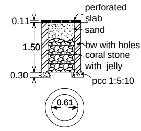
percolation pit
