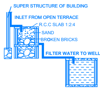
RAINWATER HARVESTING
