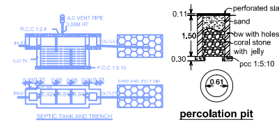
percolation pit
