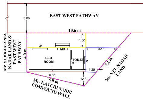
SITE PLAN (SCALE :- 1:100)
