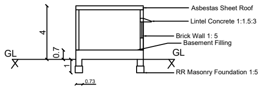
SECTION A-A VIEW
